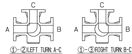
FLOW DIRECTION
