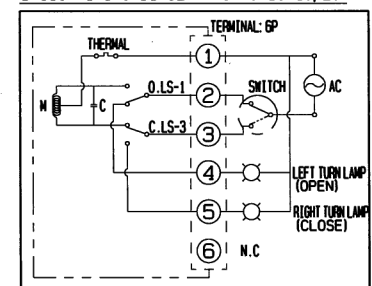
BASIC WIRING DIAGRAM FOR Unic-10, 20
